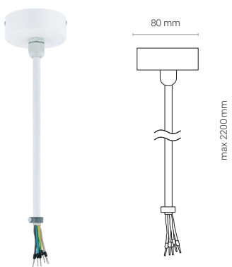
CTLS POWER SUPPLY KIT
