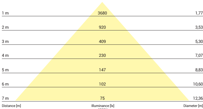
Beam cone diagram Beam angle 83°
