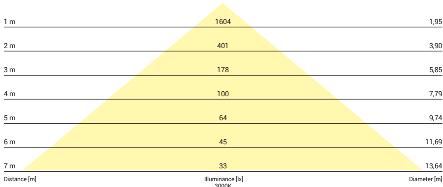
8298, 31W, 3000K, beam angle 90°
