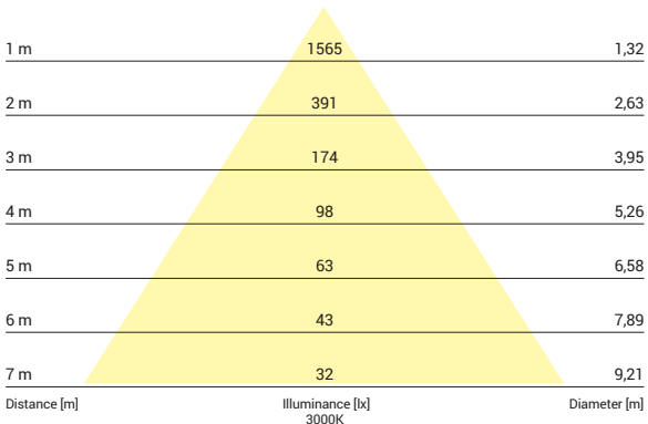
8771, 30W, 3000K, beam angle 65°
