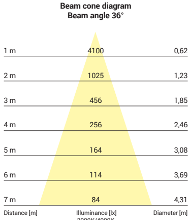
8754, 8755, 8756, 8757, 25W, 3000K, 4000K, beam angle 36°
