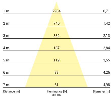
8722, 18W, 3000K, beam angle 40°
