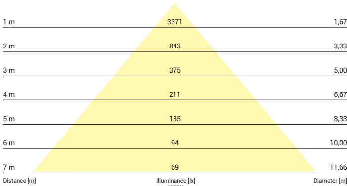
Beam cone diagram Beam angle 80°
