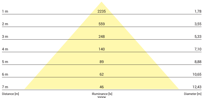
8295, 40W, 3000K, beam angle 83°
