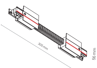
CTLS RECESSED FIXING SET
