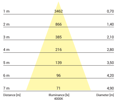
8721, 18W, 4000K, beam angle 40°
