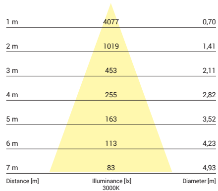
8720, 30W, 3000K, beam angle 40°
