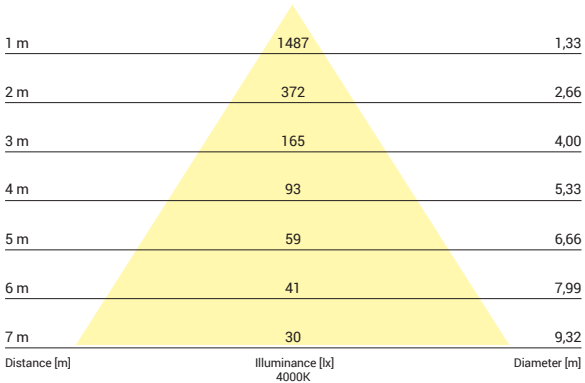
8770, 30W, 4000K, beam angle 65°
