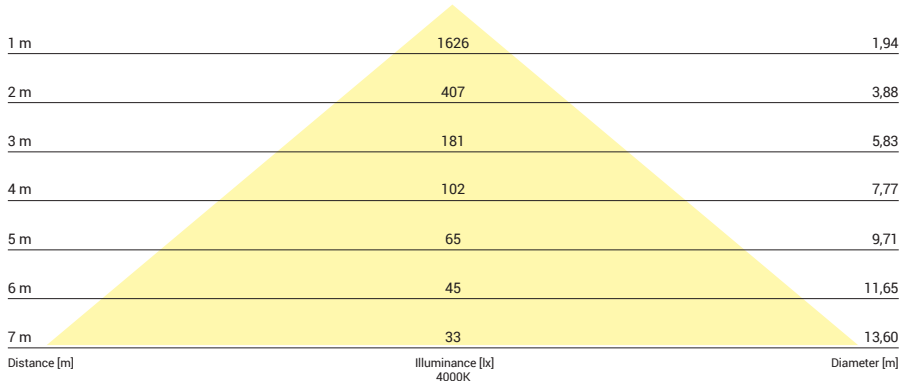
8297, 31W, 4000K, beam angle 90°
