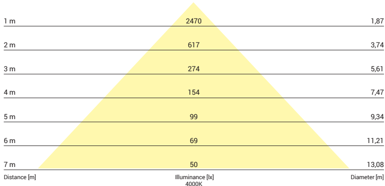
8292, 40W, 4000K, beam angle 86°
