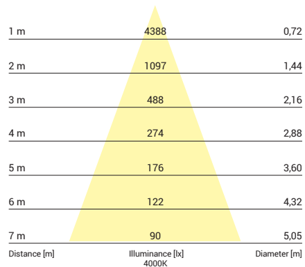
8718, 30W, 4000K, beam angle 40°
