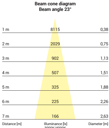
8754, 8755, 8756, 8757, 25W, 3000K, 4000K, beam angle 23°
