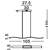
CESENA - 81002002 Chrome Aluminium & Acrylic LED 42 Watt 230 Volt 2750Lm 3000K IP20 L: 105 W: 8.5 H: 120 cm
