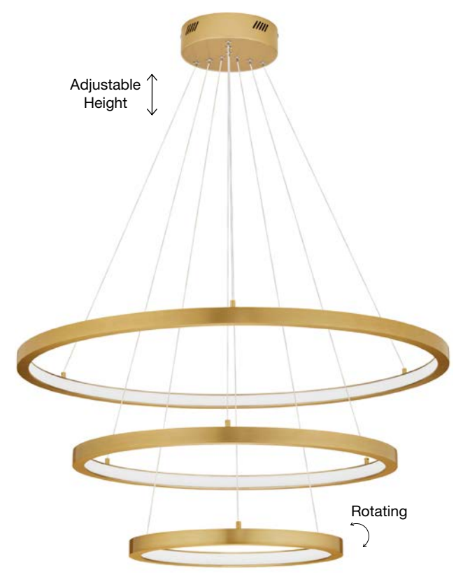
EMPATIA - 9172869 Triac Dimmable Brass Gold Aluminium & Acrylic LED 108 Watt 230 Volt 2245Lm 3000K IP20 D1: 80 D2: 60 D3: 40 H: 120 cm LED WARM WHITE DRIVER INCL.
