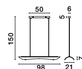
AGOS . 9054443 Triac Dimmable Gold Aluminium & Acrylic LED 34 Watt 230 Volt 2562Lm 3000K IP20 L: 98 W: 21 H: 150 cm
