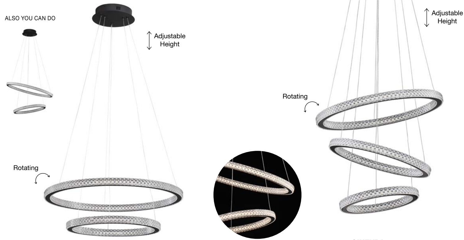
GINEVRA - 9748158 Triac Dimmable Sandy Black Aluminium & Acrylic LED 69 Watt 230 Volt 3900Lm 3000K IP20 D: 51 H: 120 cm
