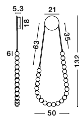
PERLA - 9695204 Triac Dimmable Gold Metal & Opal Glass LED 56 Watt 230 Volt 4734Lm 3000K IP20 L: 50 W: 5.3 H: 132 cm
