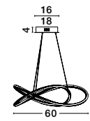
MARTINO - 8101141 Chrome Aluminium & Acrylic LED 50 Watt 230 Volt 3250Lm 3000K IP20 D: 60 H: 120 cm
