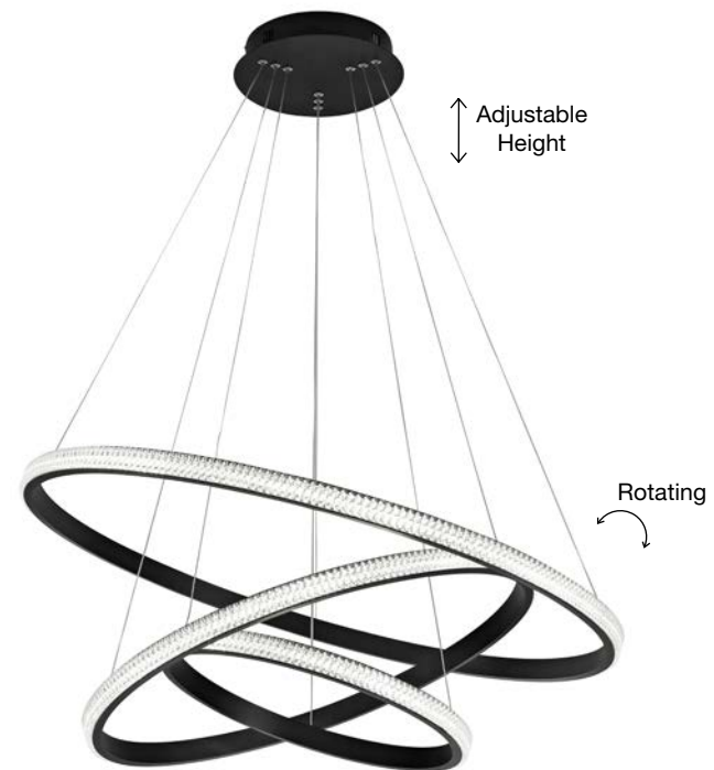
NAGER - 9481093 Triac Dimmable Sandy Black Aluminium & Acrylic LED 62 Watt 230 Volt 3586Lm 3000K IP20 D1: 78 D2: 60 D3: 41.5 H: 120 cm
