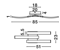
CESENA - 81002001 Chrome Aluminium & Acrylic LED 63 Watt 230 Volt 4100Lm 3000K IP20 L: 85 W: 23 H: 8 cm
