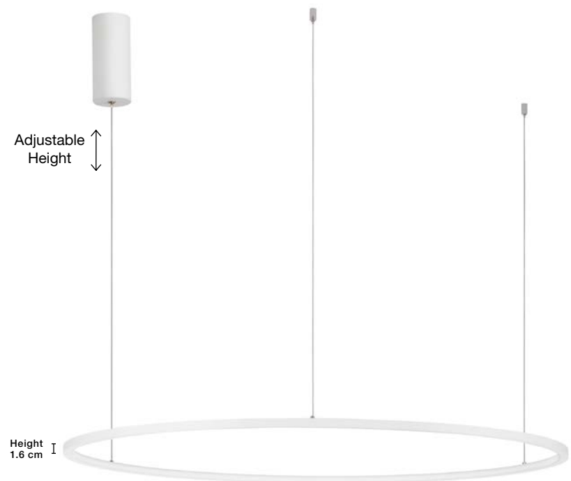
TARQUIN - 9345608 Triac Dimmable Sandy White Aluminium & Acrylic LED 59 Watt 230 Volt 2144Lm 3000K IP20 D: 100 H: 200 cm
