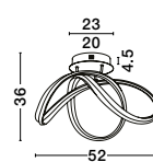
TRUNO - 9104712 Triac Dimmable Sandy Black Aluminium & Acrylic LED 60 Watt 230 Volt 4746Lm 3000K IP20 D: 52 H: 36 cm
