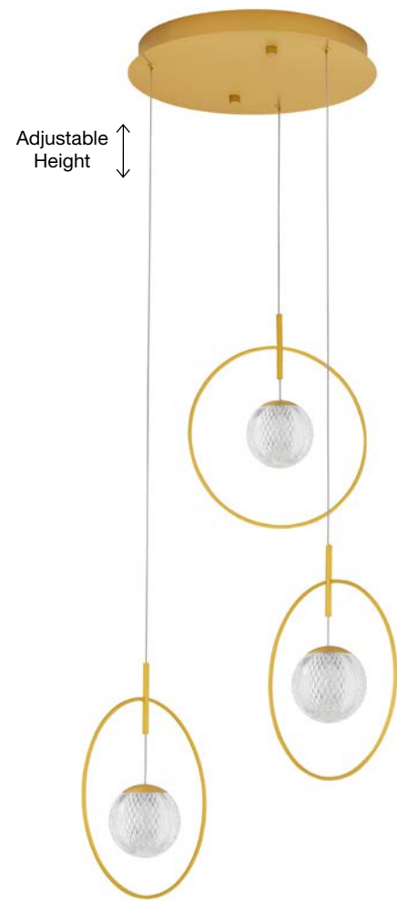
ATOS - 9695234 Satin Gold Aluminium & Acrylic LED 19 Watt 230 Volt 2208Lm 3000K IP20 D: 40 H: 200 cm
