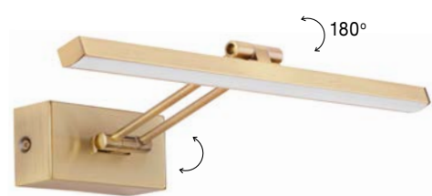
MARNELL - 9117301 Antique Brass Metal & Acrylic LED 12 Watt 230 Volt 801Lm 3000K IP20 L: 37.6 W: 20.5 H: 5.5 cm
