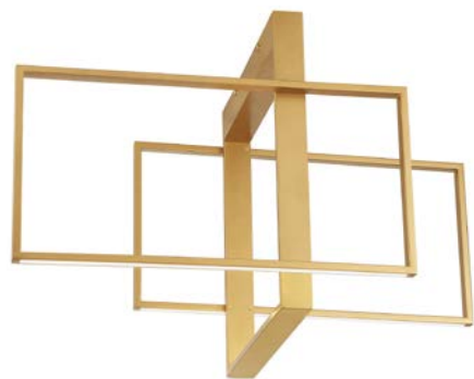
CLEA - 9086026 Gold Aluminium & Acrylic LED 26 Watt 220-240 Volt 3772Lm 3000K IP20 L: 70 W: 40 H: 40 cm
