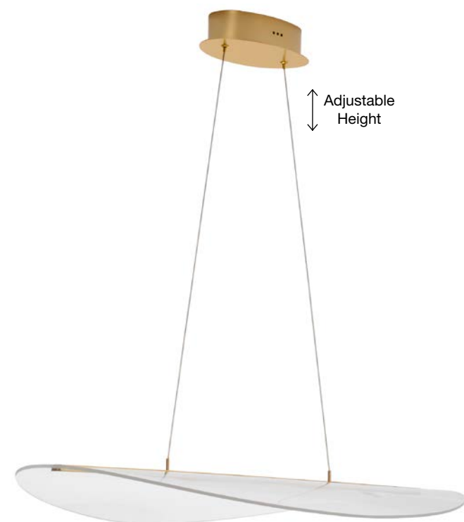
AGOS . 9054450 Triac Dimmable Gold Aluminium & Acrylic LED 32 Watt 230 Volt 2156Lm 3000K IP20 L: 95 W: 56 H: 150 cm
