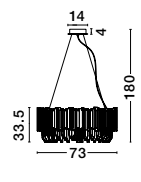
BALADONA - 81091706 Golden Brass Aluminium & Crystal LED G9 6x5 Watt 230 Volt IP20 Bulb Excluded D: 73 H1: 33.5 H2: 180 cm
