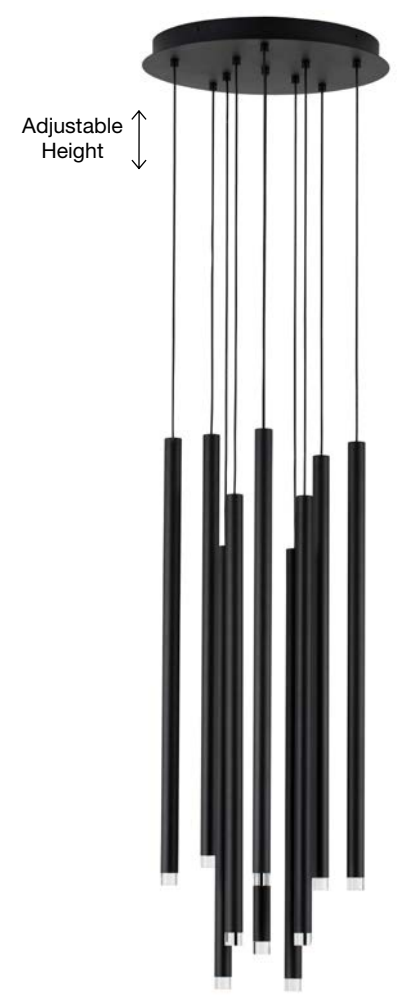
DANDIA - 9540204 Triac Dimmable Black Aluminum LED 69 Watt 220-240 Volt 4223Lm 3000K IP20 D: 40.5 H: 150 cm 40.5 40 72 150 2.8 LED WARM WHITE DRIVER INCL.
