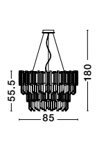
BALADONA - 81091718 Golden Brass Aluminium & Crystal LED G9 18x5 Watt 230 Volt IP20 Bulb Excluded D: 85 H1: 55.5 H2: 180 cm
