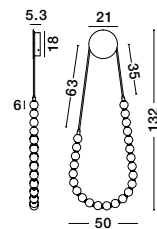
PERLA - 9186913 Triac Dimmable Chrome Metal & Opal Glass LED 56 Watt 230 Volt 4734Lm 3000K IP20 L: 50 W: 5.3 H: 132 cm
