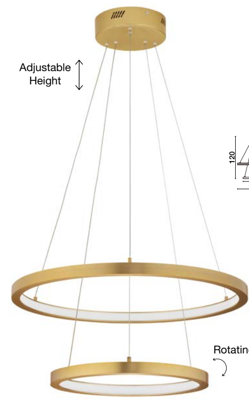
EMPATIA - 9172866 Triac Dimmable Brass Gold Aluminium & Acrylic LED 60 Watt 230 Volt 1755Lm 3000K IP20 D1: 60 D2: 40 H: 120 cm LED WARM WHITE DRIVER INCL.
