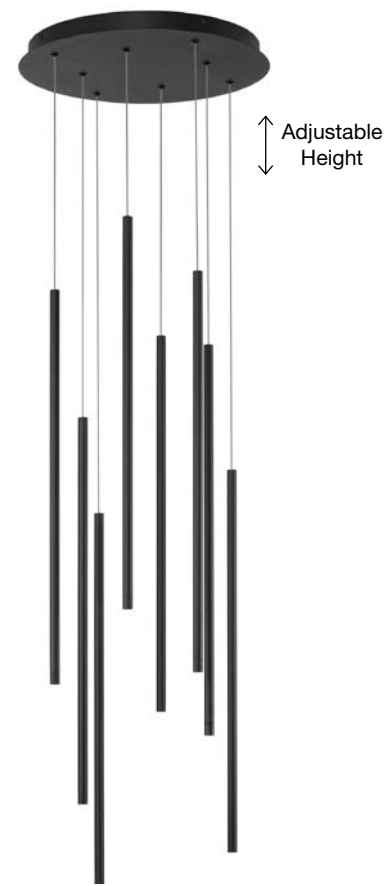
ELETTRA - 9081802 Triac Dimmable Sandy Black Aluminium LED 40 Watt 220-240 Volt 1760Lm 3000K IP20 D: 40 H: 100 cm
